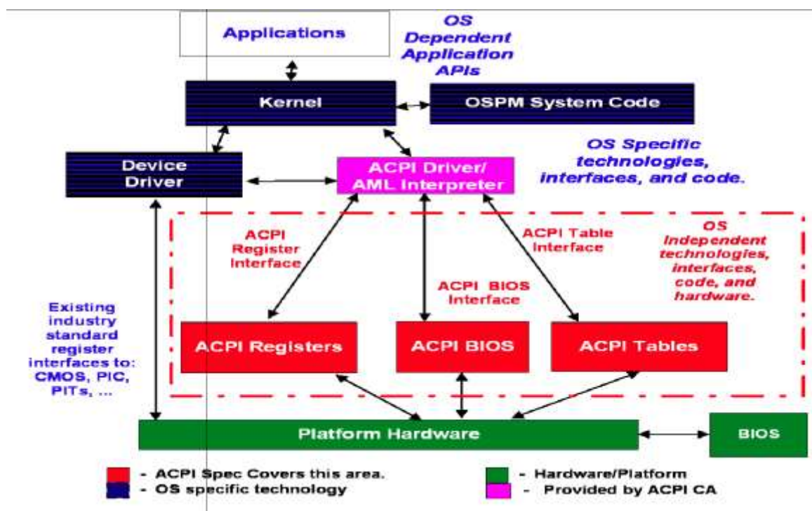
Figure 2.1 ACPI Architecture.
