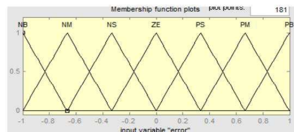
Fig.10.Membership functions
