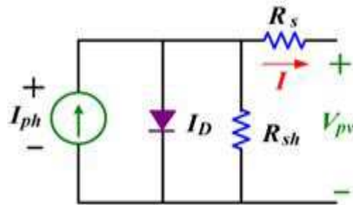
Figure 2. Equivalent electrical circuit of the PV cell.
