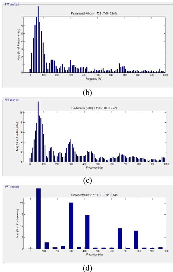
Figure 17. THD in four modes of PV system operation while utility receives power. (a) dq-current mode. (b) PV-APF mode. (c) APF mode. (d) Only utility supplies load.
