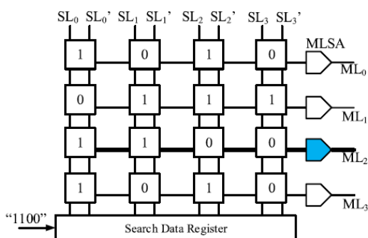
FIG. 1. EXISTED SYSTEM.
