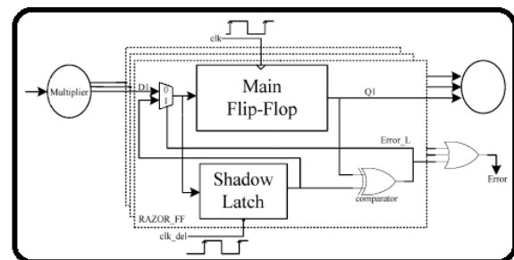
Fig.1.Circuit diagram of Razor Flip flop
