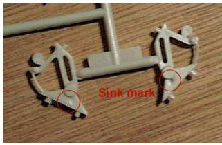
Fig. 12 Sink mark
