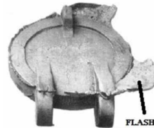
Fig. 13 Metallic projection
