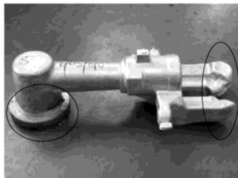
Fig. 16 Incomplete casting
