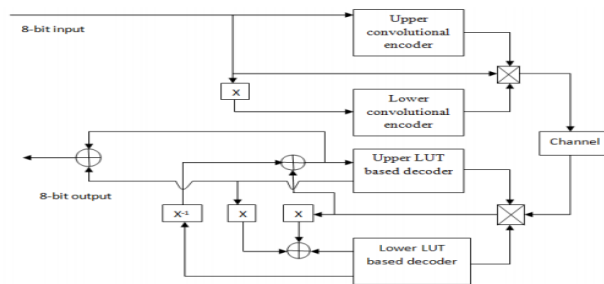
FIG.1: TURBO ENCODER AND DECODER SCHEME.
