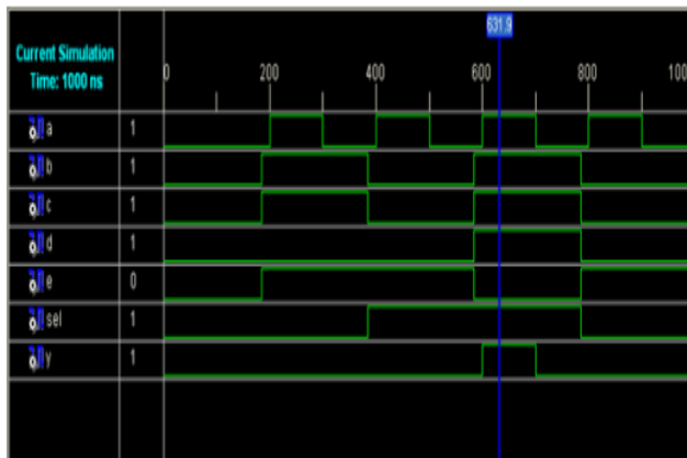
FIG.6: WAVEFORM OF ACS BLOCK.
