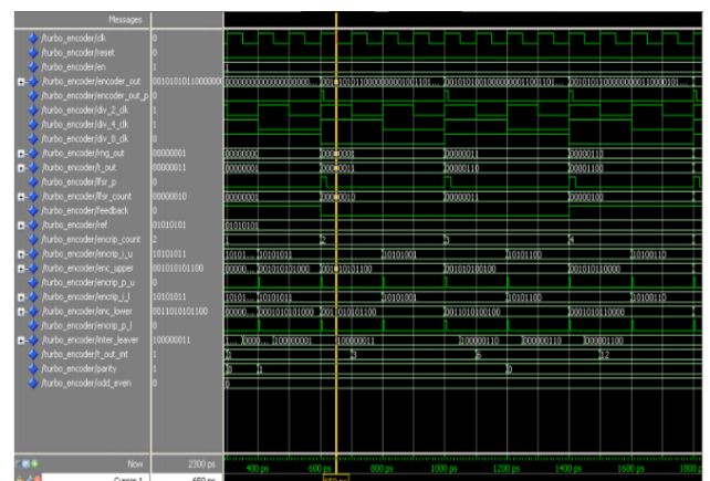
FIG.4: OUTPUT WAVEFORM OF TURBO ENCODER.
