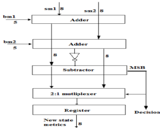
FIG.3: ACS UNIT
