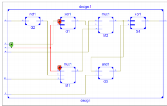
FIG.5: RTL SCHEMATIC OF ACS BLOCK.
