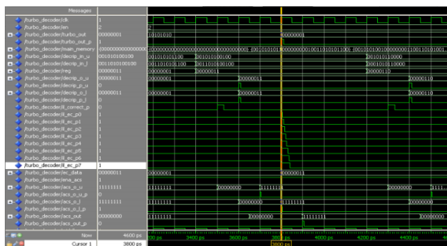
FIG.7: WAVEFORM OF THE TURBO-DECODER.
