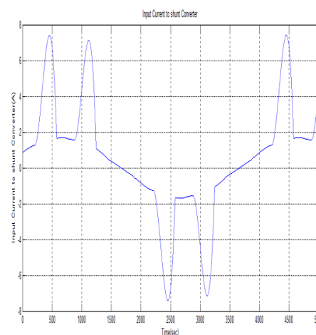
Fig. 7 Input Current to Shunt Converter
