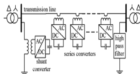
Fig. 3 DPFC configuration
