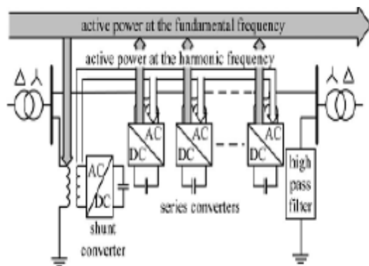
Fig.4 Active power exchange between DPFC converters
