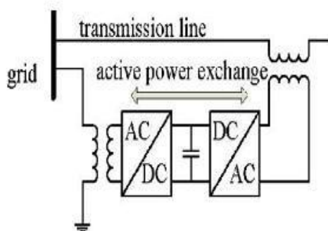
Fig.1 Simplified representation of a UPFC
