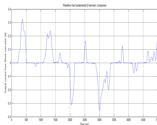
Fig. 8 Fundamental + 3 rd Harmonic Current (output voltage of Shunt converter)
