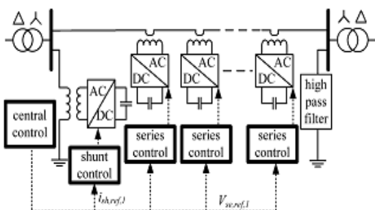
Fig. 6 DPFC control block diagram
