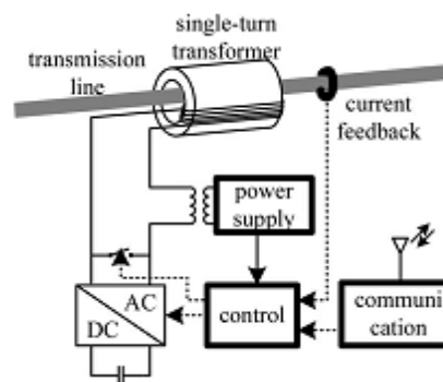
Fig.5 D-facts Concept
