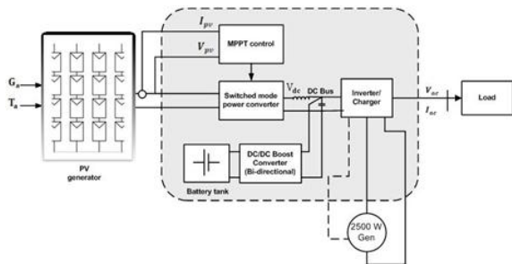
Figure 1: Hybrid stand-alone PV system
