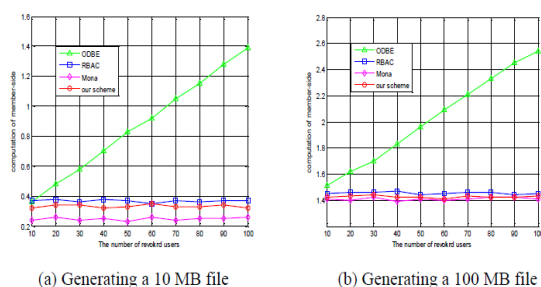
Figure 2: Comparison on computation cost of members for file upload among ODBE, RBAC
