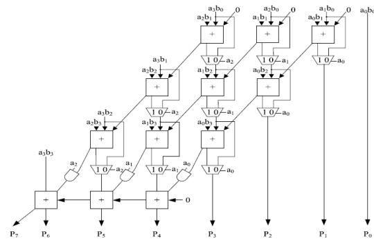
FIG.2 COLUMN-BYPASSING MULTIPLIER
