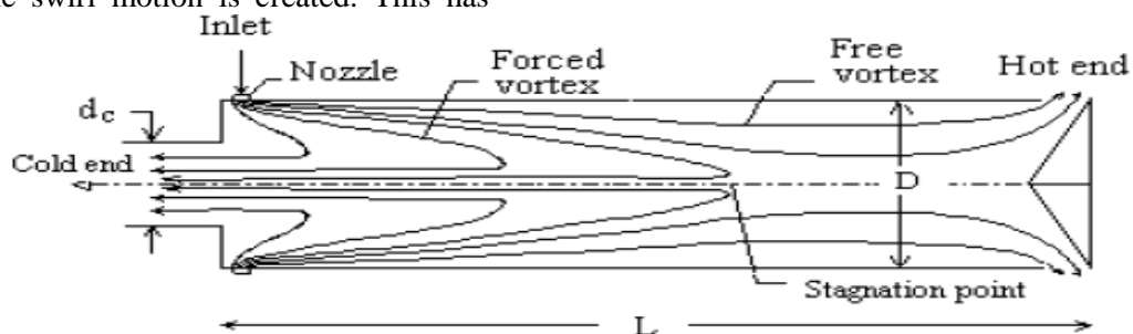
Fig: 1.2 Energy separation of counter flow vortex tube.
