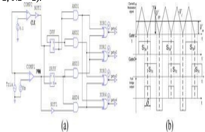
Fig. 2. Circuit and operational waveforms of symmetrical PSM. (a) Circuit of symmetrical PSM. (b) Operational waveforms of symmetrical PSM.
