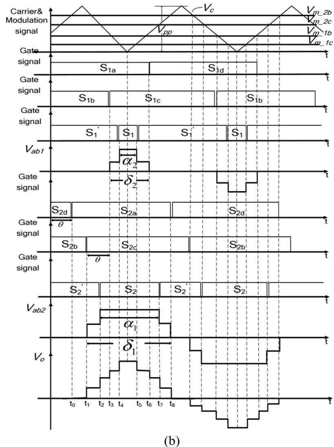
Fig.3. Operational waveforms of the proposed multilevel inverter. (a) Operational mode 1. (b) Operational mode 2.
