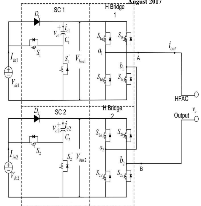
Fig. 1. Circuit topology of cascaded nine-level inverter ( M = 2, N_2 = 2 ).
