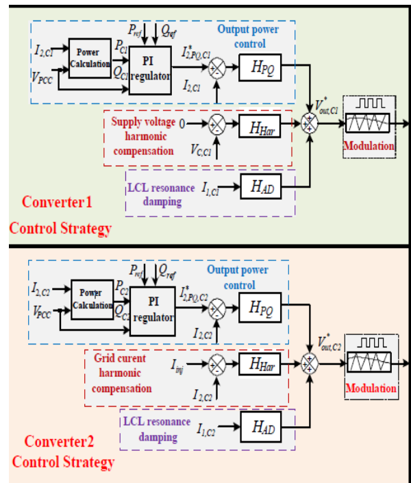
Fig. 3. Diagram of the proposed interfacing converter control strategies.
