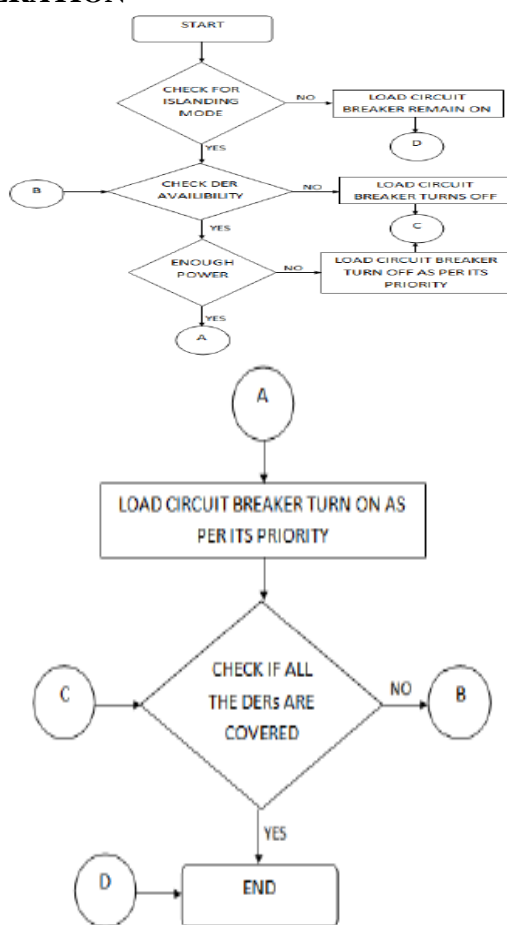
Fig. 3: Flowchart for User agent operation.
