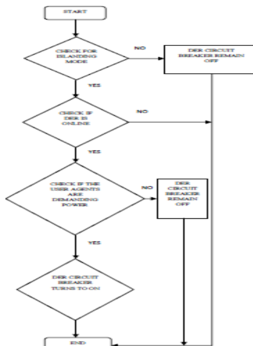
Fig. 4: Flowchart for DER agent operation.
