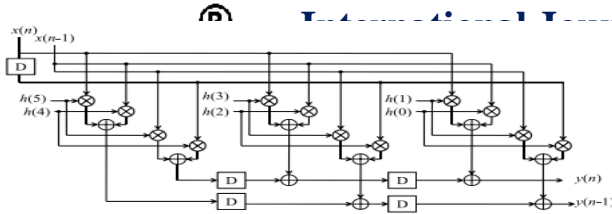
Fig. 4. Merged DFG (DFG-3: transpose form type-I configuration for block FIR structure).
