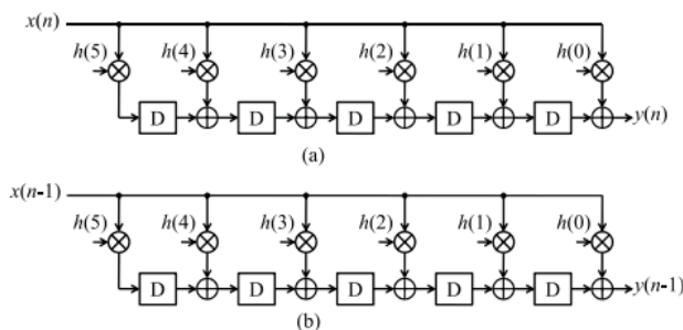
Fig. 3. DFT of DFG-1 and DFG-2 for three non overlapped input blocks [x(n), x(n - 1)], [x(n - 2), x(n - 3)], and [x(n - 4), x(n - 5)]. (a) DFT-3 for computation of output y(n). (b) DFT-4 for computation of output y(n - 1).711
