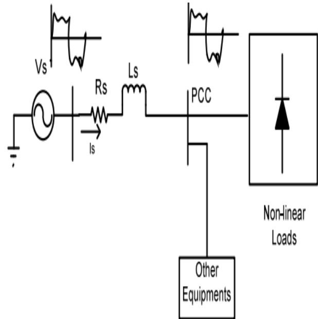
Figure.2: Power System with non-linear loads
