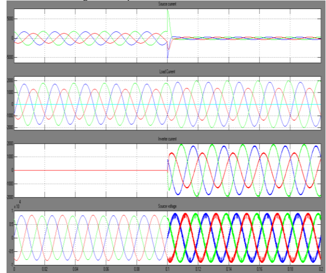
Fig.38 Source current, Load current, D-STATCOM injected harmonic current and Source voltage
