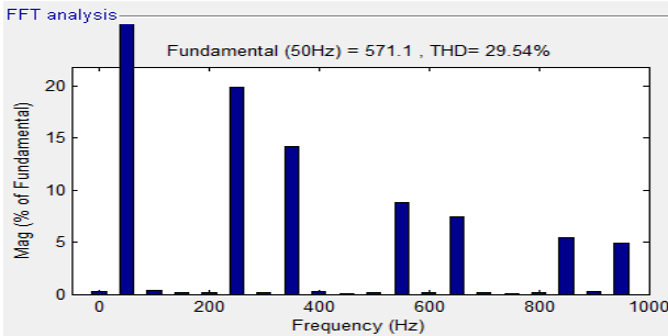
Fig.13 Load current THD
