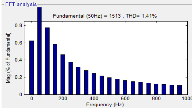
Fig.23 Load current THD
