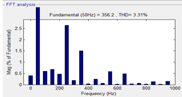
Fig.14 Source current THD
