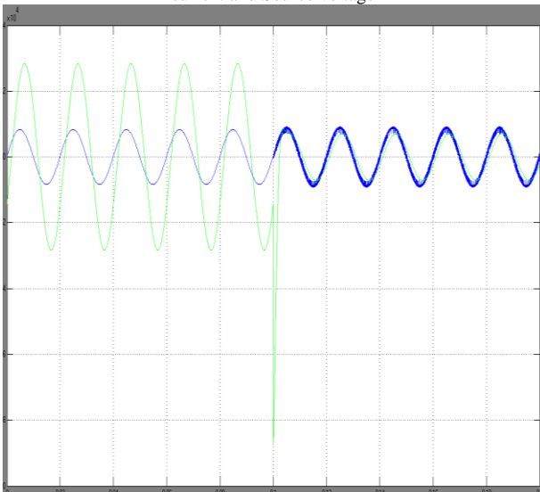
Fig.19 Power factor angle between source voltage and current
