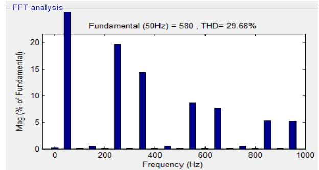
Fig.33 Load current THD
