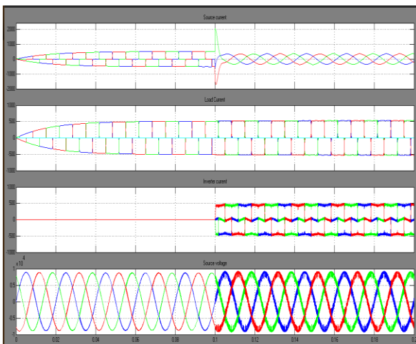
Fig.8 Source current, Load current, D-STATCOM injected harmonic current and Source voltage
