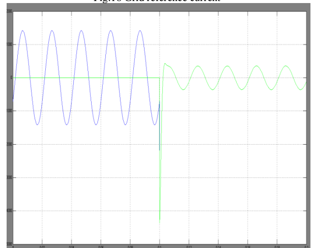
Fig.17 Grid phase and reference currents
