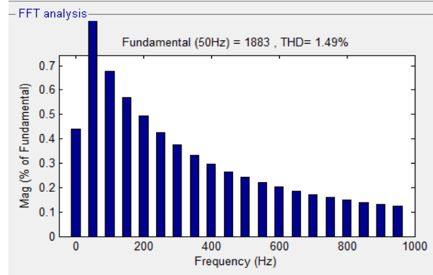
Fig.43 Load current THD
