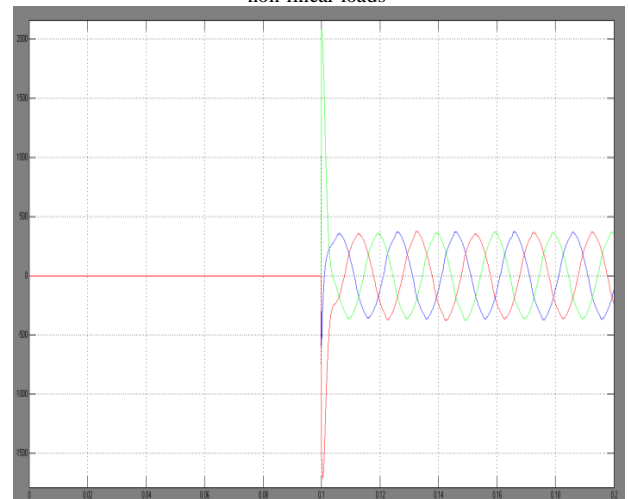
Fig.26 Grid reference current
