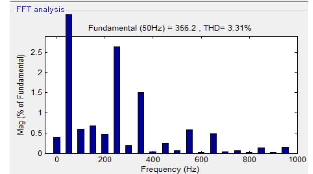
Fig.34 Source current THD
