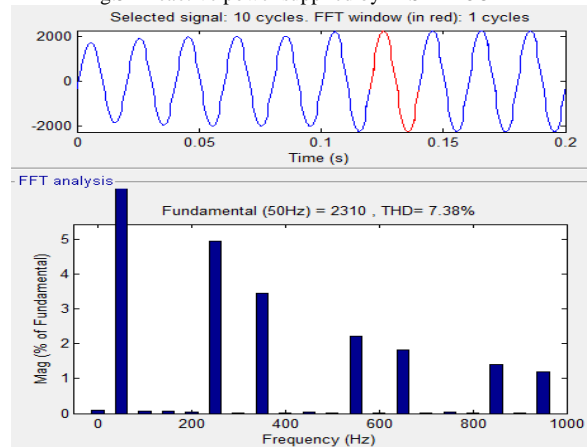
Fig.43 Load current THD
