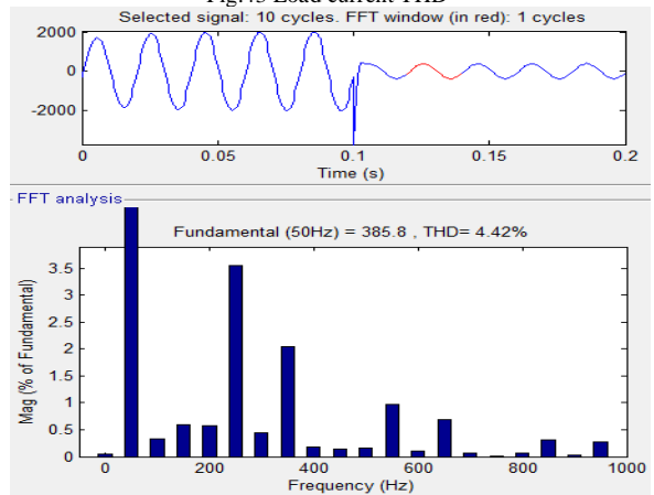
Fig.44 Source current THD
