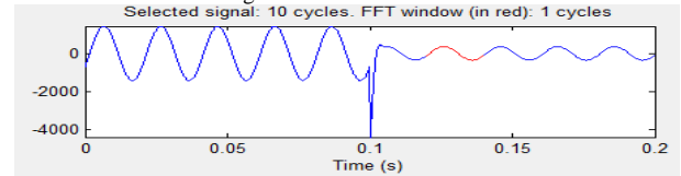
Fig.23 Load current THD
