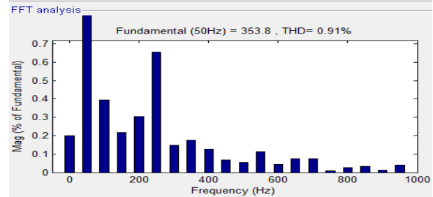
Fig.24 Source current THD
