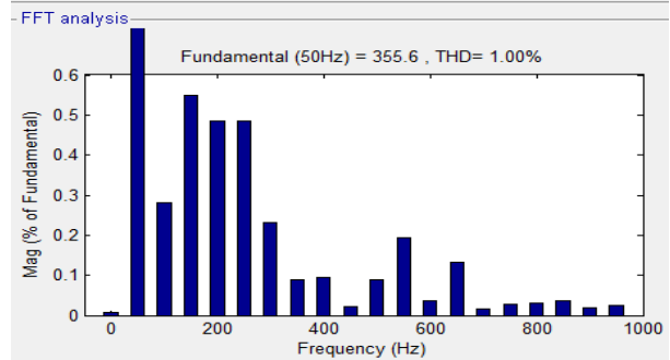
Fig.44 Source current THD
