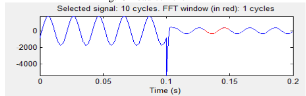
Fig.43 Load current THD
