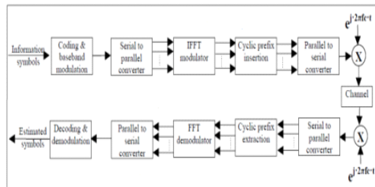
Fig.1: OFDM System
