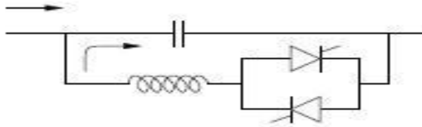
Figure 6: Vernier control mode
