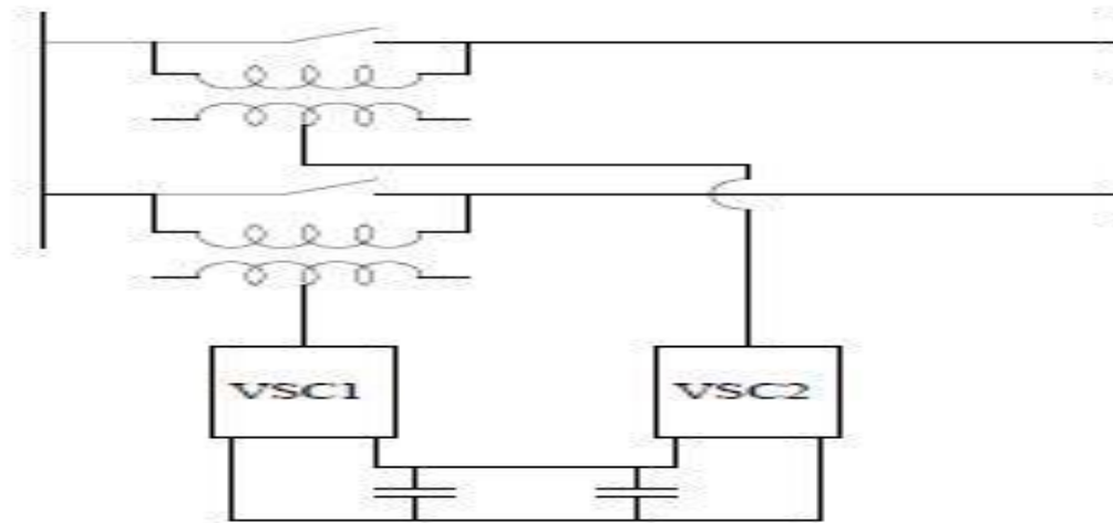
Figure 8: Unified Power Flow Controller
