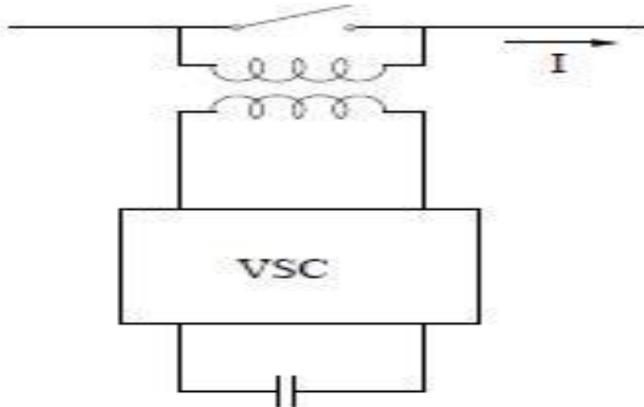
Figure 7: Static Synchronous Series Compensator
