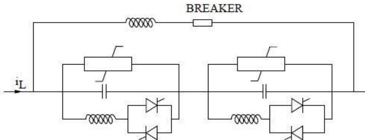
Figure 2: A Typical SVC (TSC-TCR) Configuration
