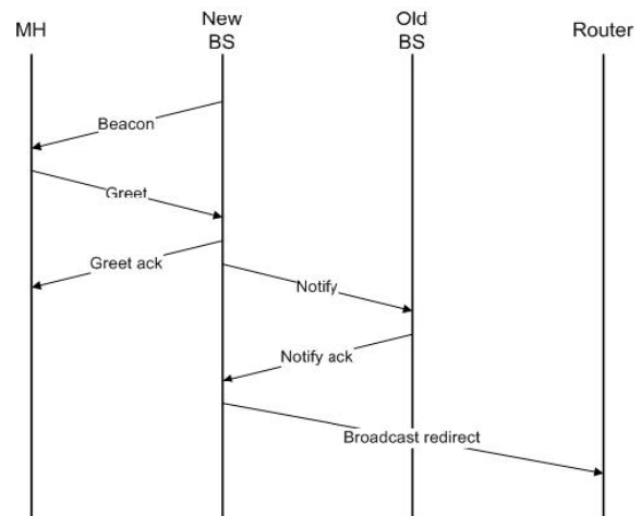
Figure 5. Enhanced ARP Handover [TTL99]
