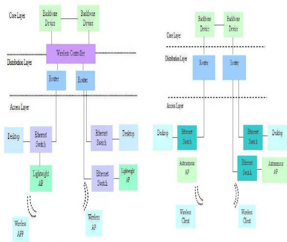
Figure2. Lightweight Architecture Model [BEM06]
