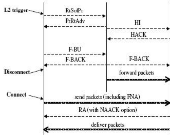
Figure 8. Fast Mobile IPv6 Handover Protocol [PaC03]
