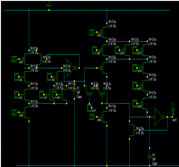
Fig.3. Schematic design of full adder circuit
