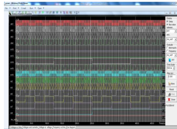
Fig.5. Waveforms of CLK and dynamic nodes of FCR cell
