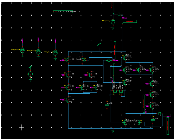
Fig.4. Schematic design of full adder with FCR circuit
