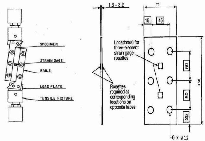
Fig: Two Rail Shear Test Method
