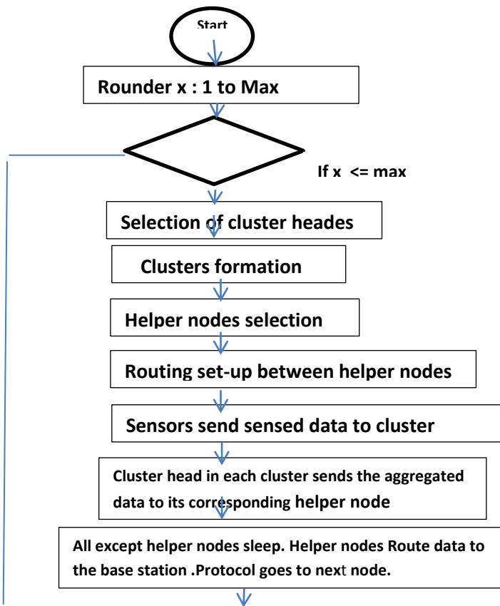
Figure 2 : Flow Chart for Operation
