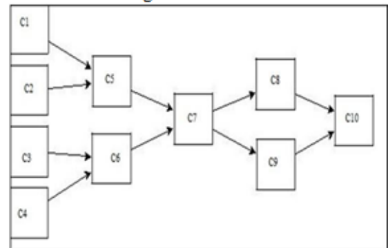
Fig1: Provenance graph
