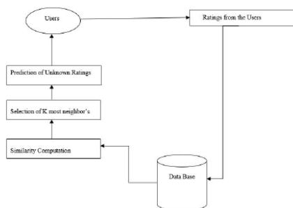
Fig. 1 Engineering of Movie recommender System utilizing Item Based Content based Filtering strategy.
