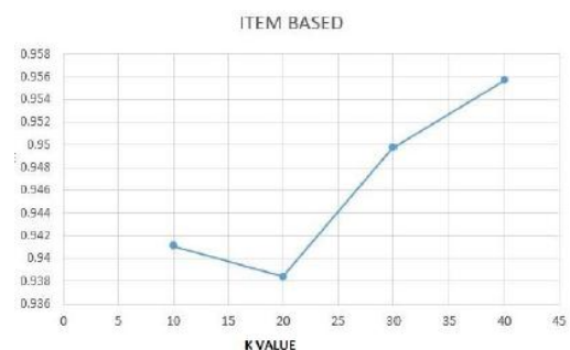
Fig. 2 Plotting of MAE for Different Values of K using item based content based filtering technique.
